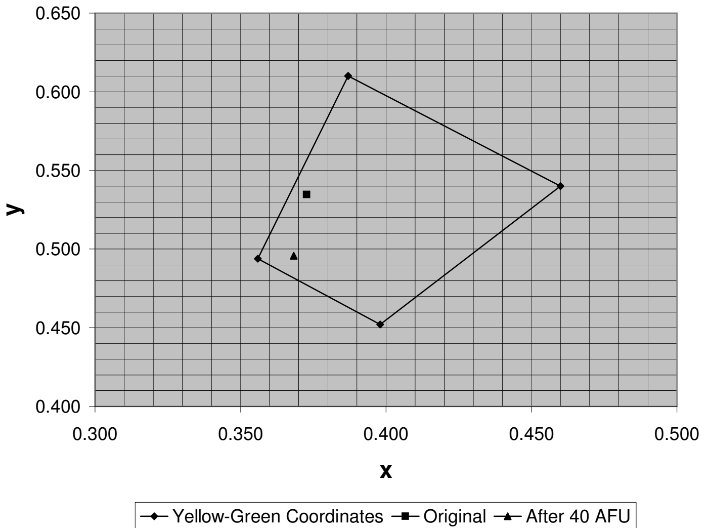
CIE 1931 (x,y) Chromaticity Diagram
